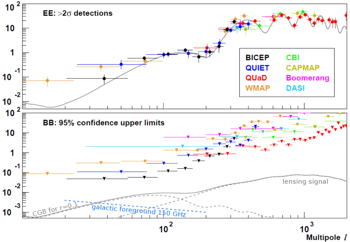
Figure 2: Current results on CMB polarization. The upper panel shows E -mode results compared to the standard \Lambda CDM expectation. The lower panel shows 95% upper limits on B -modes, with the dashed gray lines indicating B -mode signals from lensing and a possible gravity wave signal with r = 0.1 ; the solid gray line is the sum of these two signals. The dashed blue line indicates an estimate of the B -mode signal from Galactic foregrounds (both synchrotron and dust) at 150 GHz in a small, clean patch of sky. (Adapted from Chiang et al. (2009) with the addition of more recent points from the QUIET experiment and the foreground projections.)
